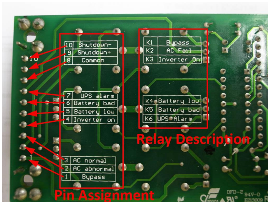
Bottom view
